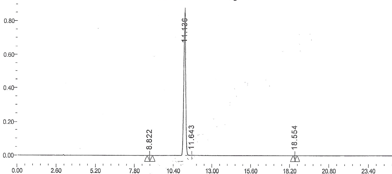
Auto-Scaled Chromatogram
